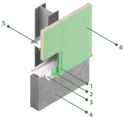
07 Drip Flashing Detail
