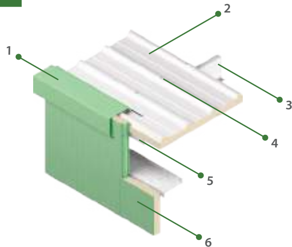
10 Gable Detail
